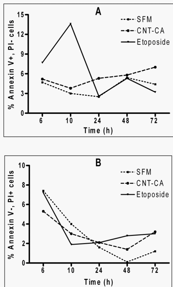
Fig. 2. Analysis of the effects of CNTs on cell state by flow cytometry. NS1 cells were treated with SFM, CNT-CA or etoposide, double-stained with annexin V-FITC and PI and analyzed by flow cytometry. Panel 2A represents the scatter plots at 10 h (A-C) and 24 h (D-F) exposures to SFM (A, D), CNT (B, E) and etoposide (C, F). The line graphs in panel 2B represent the time course of generation of early apoptotic (A), or necrotic (B) cell populations in cells treated with SFM (○), CNT-CA (*), or etoposide (▲).
